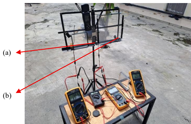
Gambar 5 Visualisasi proses pengujian lapangan, (a) Sampel 1 LSC-PV 10 cm × 10 cm (b) Sampel 2 LSC-PV 20 cm × 20 cm.
