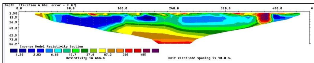
Figure 5. Results of processing data from line 1
