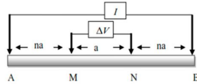
Figure 4 Wenner Schlumberger configuration
