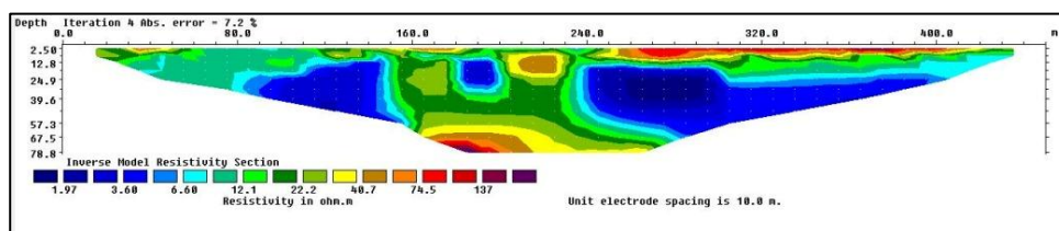
Figure 8 Results of processing data from line 4
