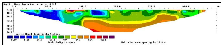
Figure 6. Results of processing data from line 2
