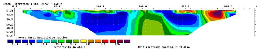
Figure 9 Results of processing data from line 5
