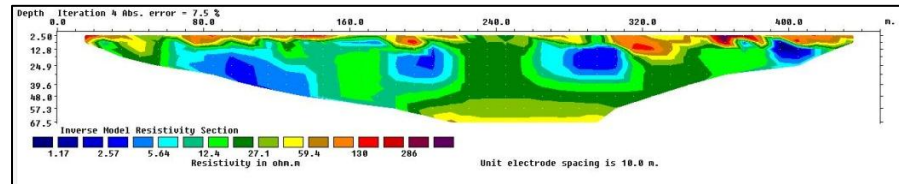
Figure 7 Results of processing data from line 3
