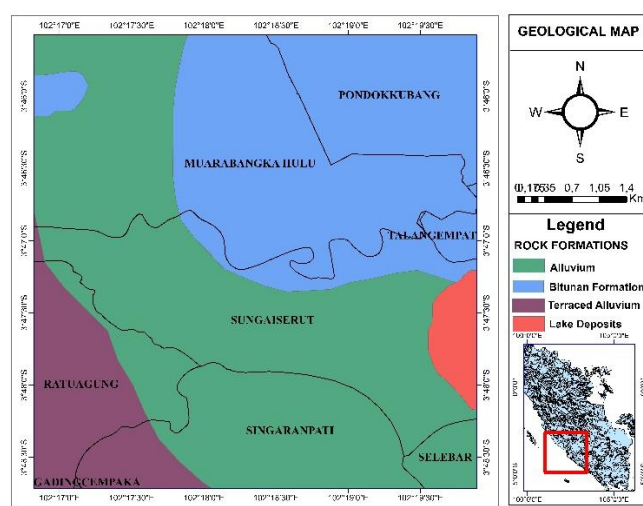
Figure 1. Geological map of Bengkulu City (Gafoer et al., 2007)
